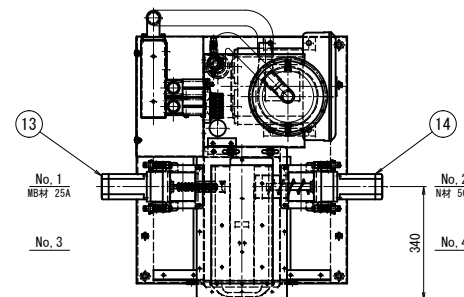
View from B-B B-B矢視
