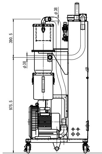
View from A A矢視
